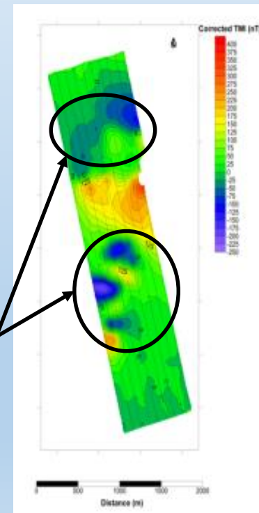
Magnetic Map After Compensation
