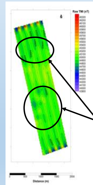
Magnetic Map Before Compensation
