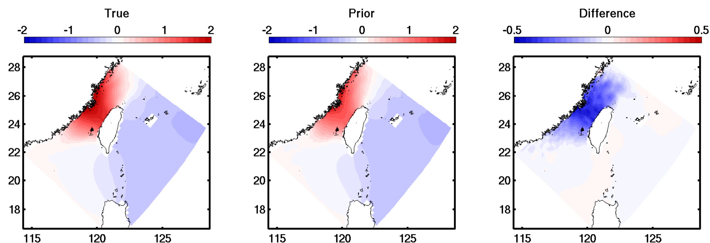
Figure 2: Modeled Sea Surface Height. Tidal SSH computed from S&S v12.1 (left) is visually similar to ETOPO2v2 (middle), except for the reduced tidal amplification in the Strait of Taiwan. The difference field (right) is used to reconstruct the bottom topography. Units of SSH are meters.
