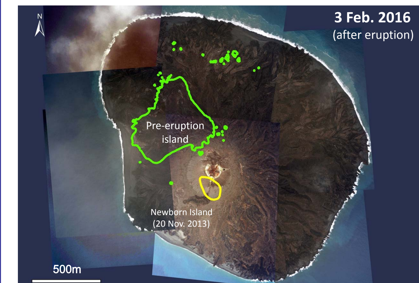
Fig.7 Change of Nishi-no-shima Island during the 2013-2015 eruption
