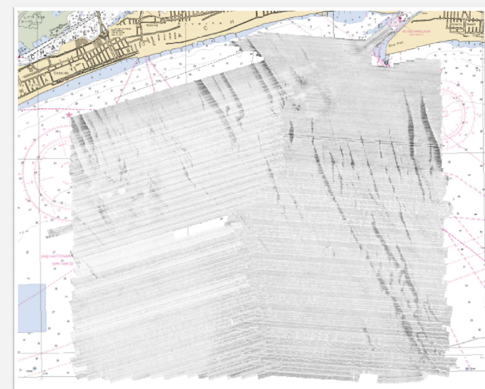
Fig. 2 An example of project product. Side Scan Sonar mosaic, with 1m resolution, 200% coverage, generated from H12138 survey data, displayed over the nautical chart No. 12305.
